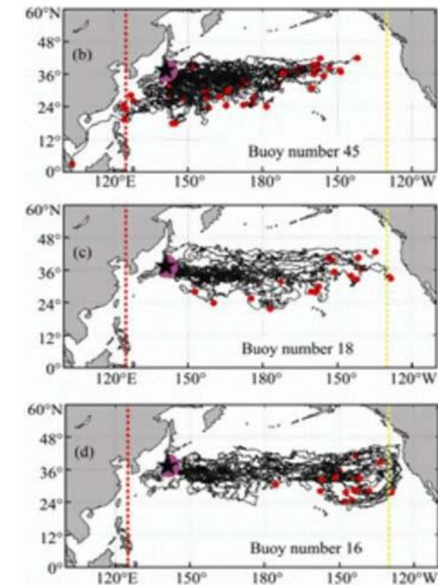
The black lines and red dots represent trajectories and terminal positions of the surface drifters originated from the source region with the lives of (b), 2–3 years (c), more than 3 years (d), respectively.
