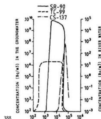
(Above) Radionuclide concentrations in groundwater and river water - X axis represents days since the initial meltdown ( 10^3 = 1,000 days; 10^4 = 10,000 days; 10^5 = 100,000 days)
