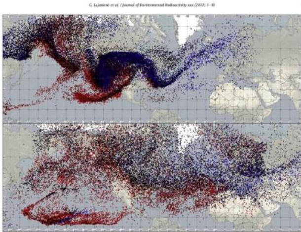
339 (Above) Fig. 1. Particles spacing on 20 March, 2011 at 12:00 UTC (top) and on 27 March, 2011 at 18:00 UTC (bottom); shades of red indicate particles in the bottom layer, up to 3 km; black to dark blue indicate the middle layer, up to 6 km height; and light blue indicates the upper layer; the trajectories were simulated using the Lagrangian dispersion model (time of the particles release was on 12 March 2011). (For interpretation of the references to colour in this figure legend, the reader is referred to the web version of this article .)
