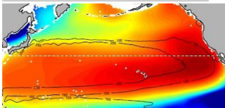
(Above) Subsurface concentration of Cs-137 (Bq/m3) at 150-250m (Rossi et al 2013)
