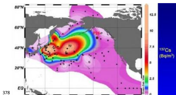
(Above) Surface water distribution of Fukushima 137Cs in 2012
