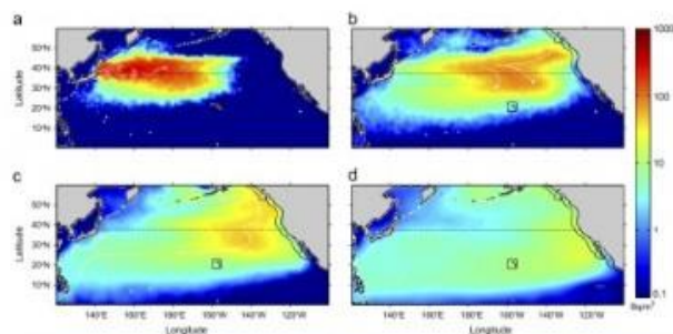
Surface (0-200m) of Cesium-137 concentrations (Bq/m 3 ) by (a) April 2012, (b) April 2014 (c) April 2016 and (d) April 2021 — Hawaii seen in black square (SOURCE: Rossi, et al.)
