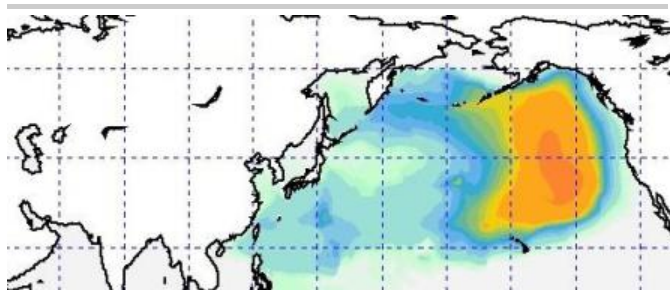
(Above) Model produced by governments of Korea and China
