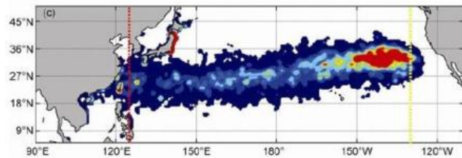
(Above) Impact strength of Cs-137 in year 4 (Han G J, et al. 2013)
