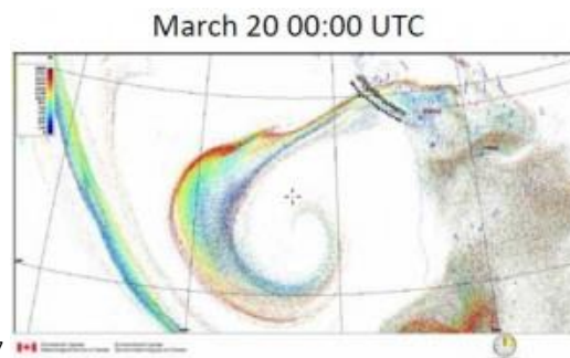
(Above) land map is removed from study images. For reference, row of dots in the upper right denote monitoring stations along Vancouver Island coast.
