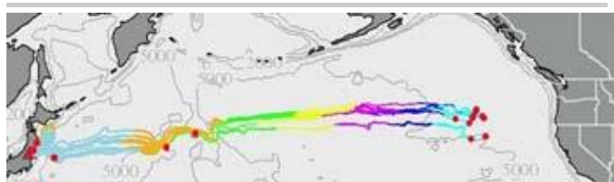
(Above) Model produced by governments of Korea and China
