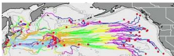
(Above) Top: 200 meters; Bottom: 50 meters, variable depth (Z. Lai et al.)
